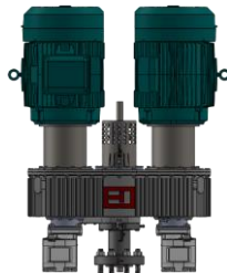
Dual Motor gear drive 75-250hp
